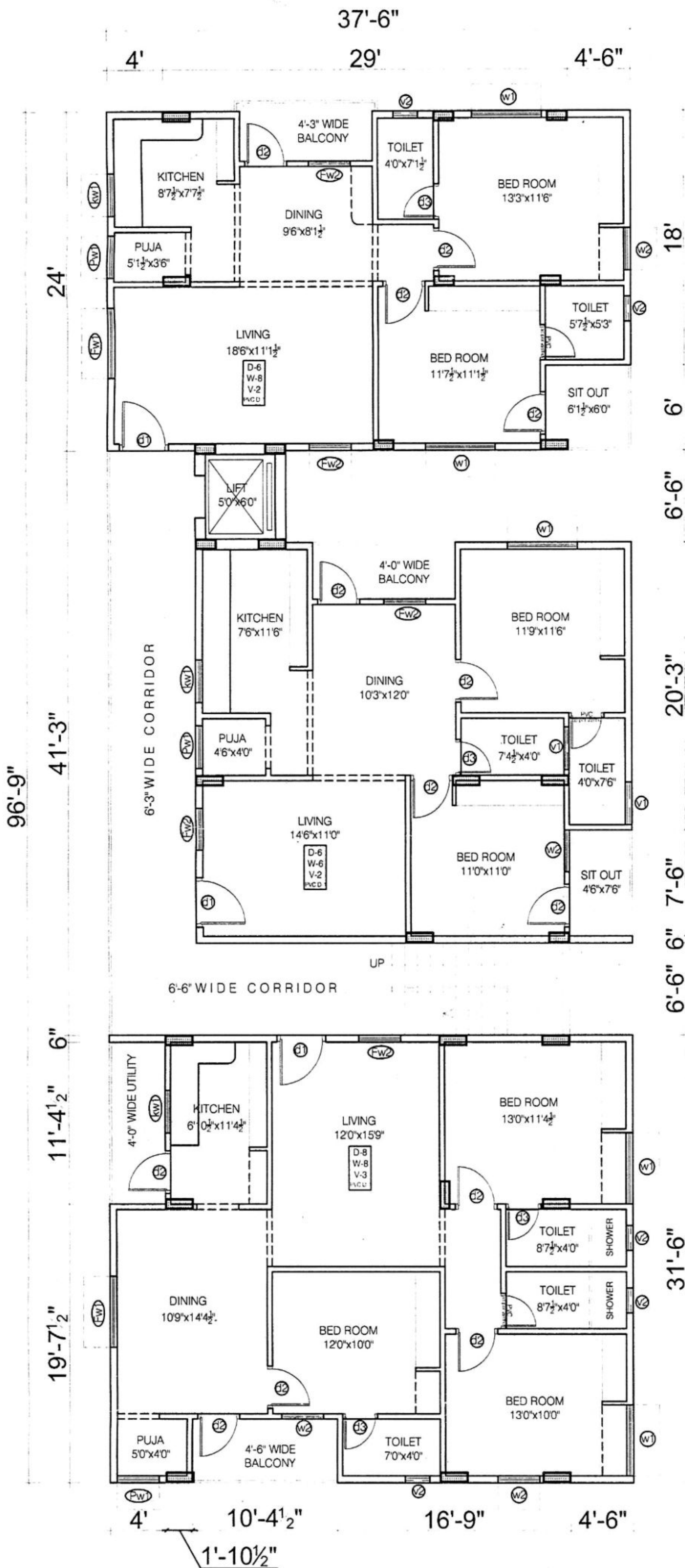
TYPICAL FLOOR PLAN
